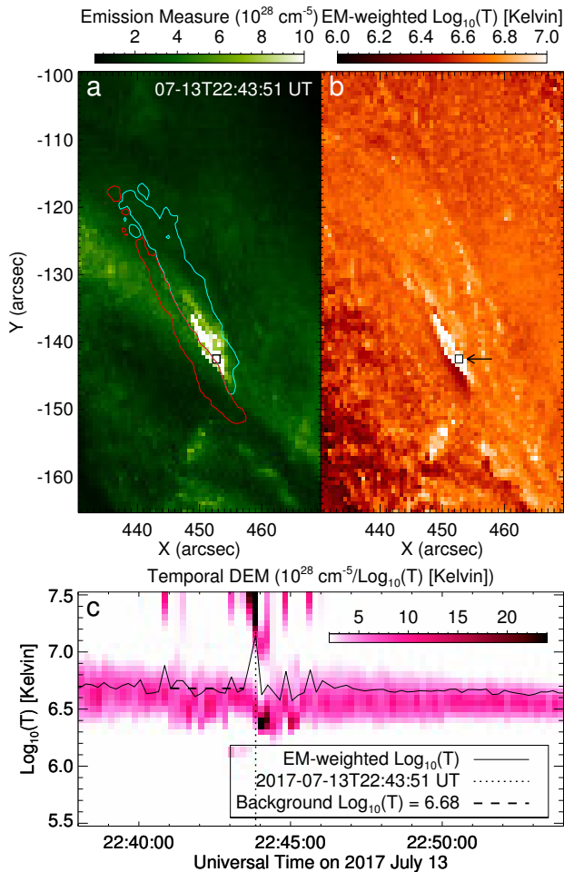
Figure 4. Differential emission measure (DEM) and emission measure (EM) of the reconnection region based on SDO/AIA observations. (a) The EM that is the zeroth moment of DEM. (b) The EM-weighted temperature which is the first moment of DEM divided by EM. (c) The temporal changes in the DEM that is averaged over the four pixels specified by the square in (b). The field of view of (a)-(b) is similar to that of Figure 2(c)-(e). The contours in (a) are the same as those in Figure 2(b). In (c), the solid curve is the EM-weighted temperature corresponding to the DEM, the dashed line denotes the averaged background EM-weighted temperature (with its span representing the time range 22:41:03 – 22:43:27 UT), and the dotted line marks the peak time of the EM and EM-weighted temperature.
